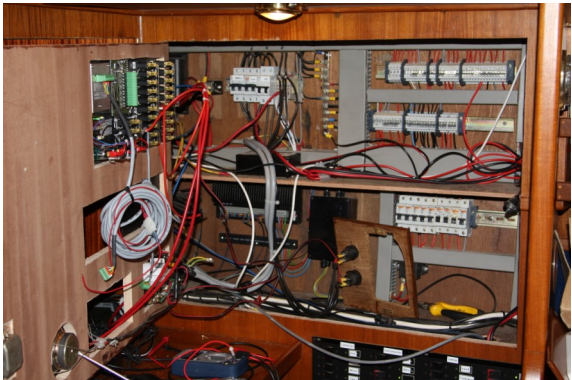
Rewired all electrics and new electronics
